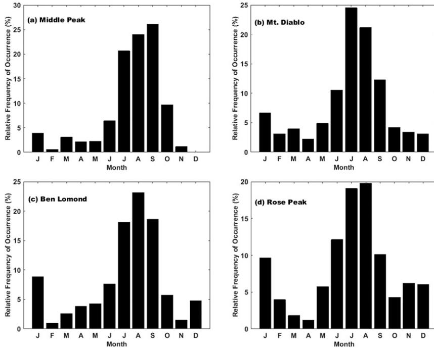
FIG. 6. Relative frequency of occurrence (%) by month when RH < 9.5\% and DP \leq -10^\circ\text{C} for (a) Middle Peak, (b) Mount Diablo, (c) Ben Lomond, and (d) and Rose Peak between 2000 and 2014.
