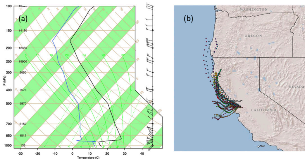
FIG. 4. (a) KOAK upper-air sounding from 0500 PDT 29 Aug 2003 of temperature (black), dewpoint (blue), and wind barbs ( \text{m s}^{-1} ), and (b) 24-h 27-member HYSPLIT backward trajectories from the time of the Devil Fire shelter deployment site.
