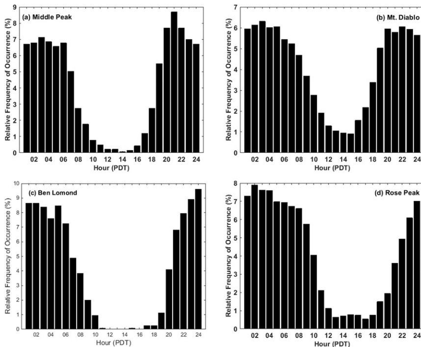
FIG. 7. As in Fig. 6, but for relative frequency of occurrence (%) by hour (PDT).
