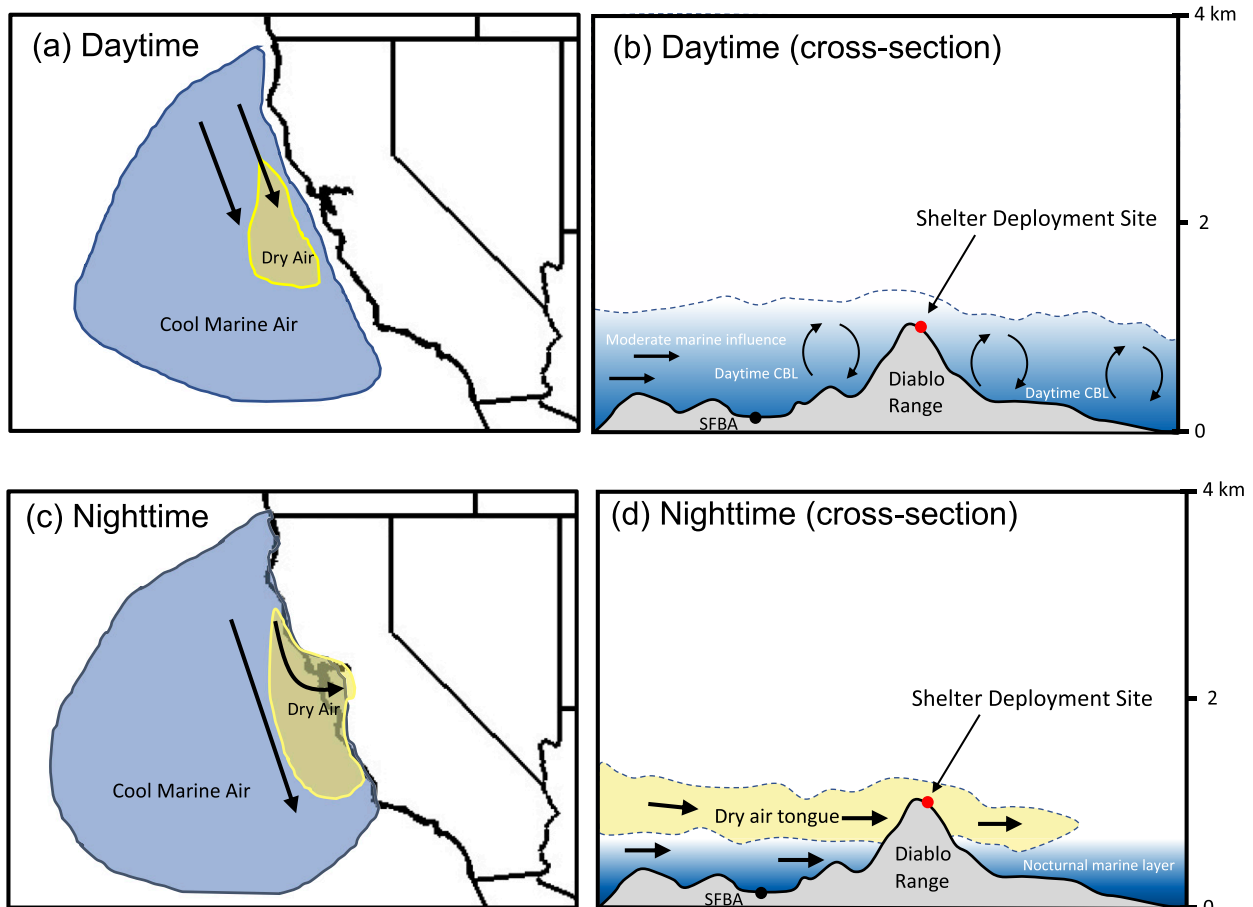
FIG. 15. Conceptual model of NDEs and their diurnal evolution. Blue shading represents cool, moist marine air, and yellow shading represents warm and dry air aloft. Arrows are generalized wind vectors. The SFBA and shelter deployment site are shown.
